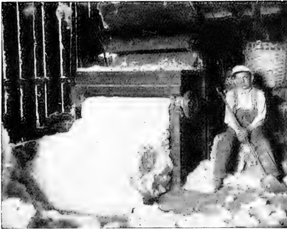
FIG. 63.—Inside view of ginnery, showing sheet of loose cotton lint as it comes from the cotton gin, just before baling.
